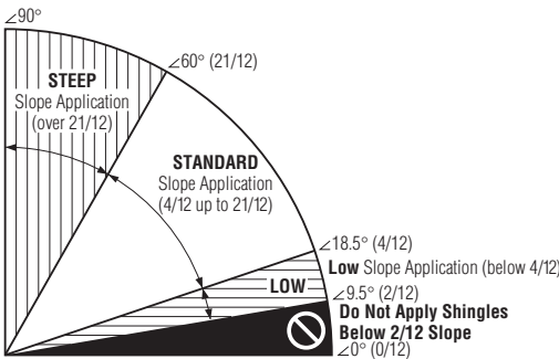
Figure 17-2: Slope definitions.
